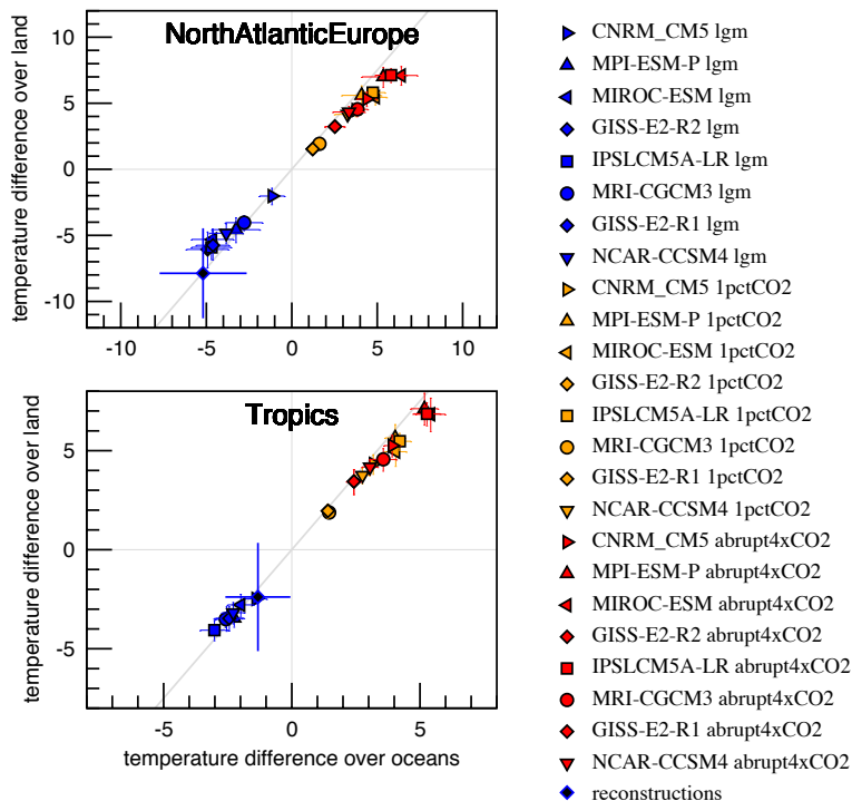
Fig. 2. Average surface air temperature change, compared to piControl, over land compared to over the oceans for the North Atlantic and Europe region (45° W–45° E, 30°–50° N) and the tropics (23° S–23° N). LGM – piControl in blue, 1pctCO2 – piControl in orange, abrupt4xCO2 – piControl in red. For the latter 2 periods, the averages have been computed over the same years as Fig. 1 above. The results have been computed for all models in the database on 23 July 2012 for which there were results for the lgm, piControl, 1pctCO2 and abrupt4xCO2. The grey lines indicate the 1 : 1.5 ratio in both plots. Reconstructions are as in Fig. 1.
