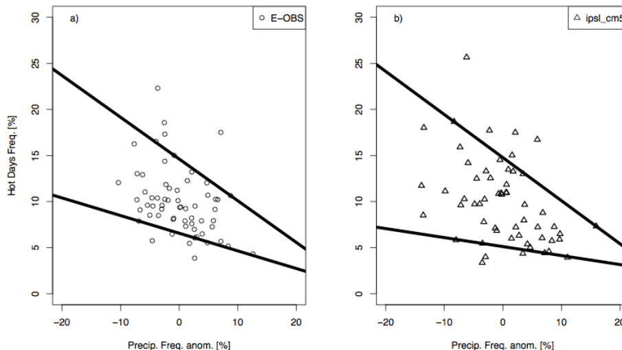
Fig. 3. Illustration of quantile regressions between the percentage of summer hot days in Europe (i.e. exceeding the 90th quantile of daily mean temperature in June–July–August) and the precipitation frequency anomaly with respect to the mean in winter–spring (January to May). The precipitation frequency is computed over southern Europe ( 36^{\circ} N to 46^{\circ} N) and is defined as the percentage of days with precipitation exceeding 0.5 mm. The quantile regressions are computed for the 10th and 90th quantiles of the hot day frequency, following Quesada et al. (2012). (a) shows the quantile regression for Western Europe from the EOBS dataset (Haylock et al., 2008) between 1950 and 2011 where each point represents a year. (b) is for the “historical” simulation (1960–2008) of the IPSL-CM5A-MR model (Dufresne et al., 2013). Both panels show a widening of the quantile regression for low values of precipitation frequency, indicating a consistency of the model simulation with observations.
