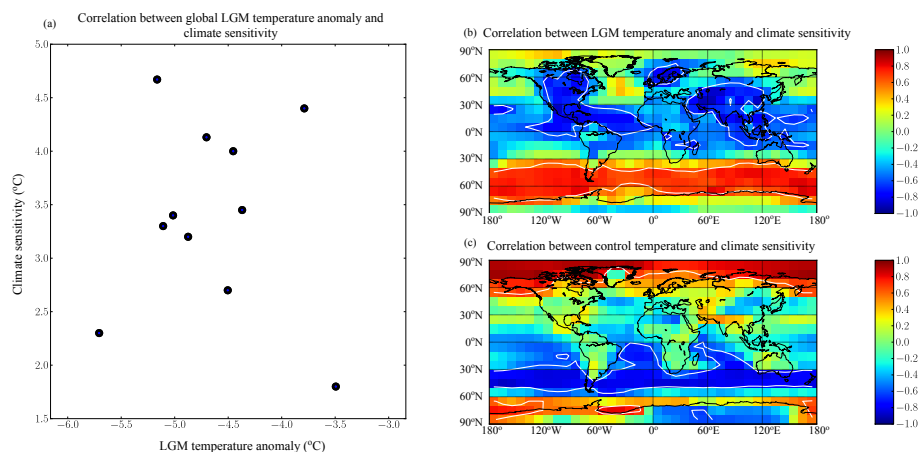
Fig. 5. (a) Global mean LGM temperature change versus overall climate sensitivity to 2\times\text{CO}_2 . (b) Correlation between local air temperature anomaly and climate sensitivity across the model ensemble. (c) Correlation across the model ensemble between control run temperatures and climate sensitivity.
