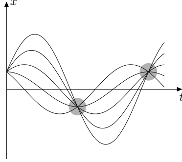
Fig. 7. In a harmonic potential all trajectories emerging from the same starting point converge at conjugate points at multiples of half an oscillation period
