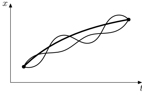
Fig. 2. The thick line represents a classical path satisfying the boundary conditions. The thinner lines are no solutions of the classical equation of motion and may be associated with quantum fluctuations
