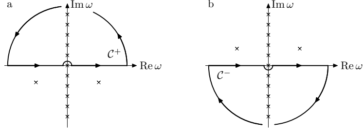
Fig. 12. The analytic continuation of the imaginary time correlation function \langle q(\tau)q(0) \rangle to real times makes use of the integration contours depicted in (a) and (b) to obtain (217) and (218), respectively
