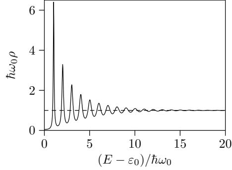
Fig. 11. The density of states (197) of the damped harmonic oscillator is shown for \gamma/2\omega_0 = 0.05 . A delta function contribution at E = \varepsilon_0 has been omitted. The dashed line marks the average density of states 1/\hbar\omega_0
