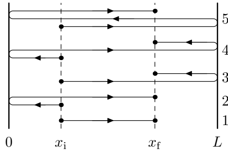
Fig. 4. The reflection at the walls of a box leads to an infinite number of possible trajectories connecting two points in the box
