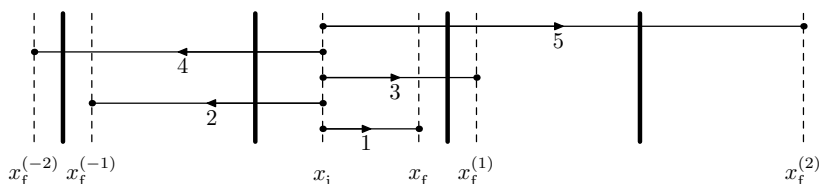
Fig. 5. Instead of a particle getting reflected at the walls of the box one may think of a free particle moving from the starting point in the box to the end point in one of the replicas of the box
