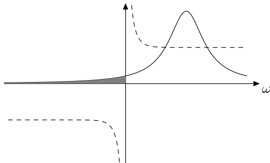
Fig. 13. The full and dashed lines represent the Lorentzian and hyperbolic cotangent, respectively, which contribute to the integrand in (238)
