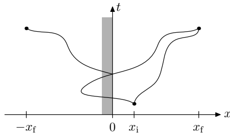
Fig. 6. A path crossing the wall is cancelled by a path running to the mirror point of the end point
