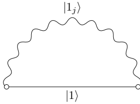
Fig. 10. The ground state energy of the harmonic oscillator is shifted by a transition to the first excited state accompanied by a virtual excitation of the j -th environmental mode
