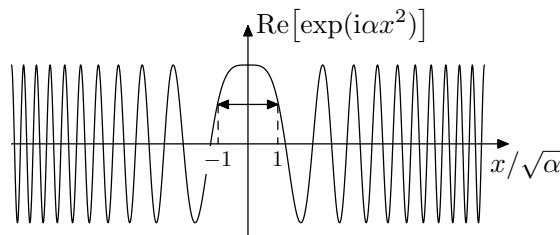
Fig. 8. In stationary phase approximation only a small region around the extremum contributes to the integral. For the example shown here, the extremum lies at x = 0
