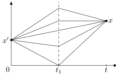
Fig. 1. According to the semigroup property (9) the propagator K(x, t, x', 0) may be decomposed into propagators arriving at some time t_1 at an intermediate point x'' and propagators continuing from there to the final point x
