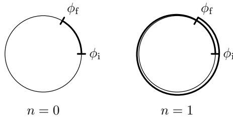
Fig. 3. On a ring, the angles \phi_f and \phi_f + 2\pi n have to be identified. As a consequence, there exist infinitely many classical paths connecting two points on a ring, which may be identified by their winding number n
