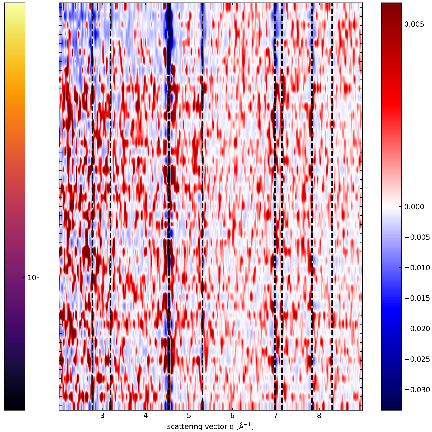
lineouts difference
